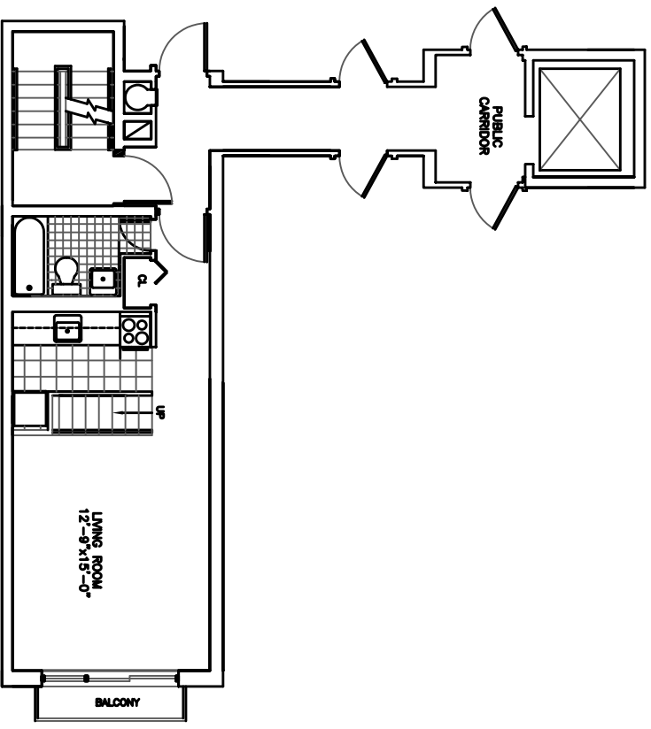
UNIT C 128 EAST 85TH STREET, 8TH FL (LOWER LEVEL)
